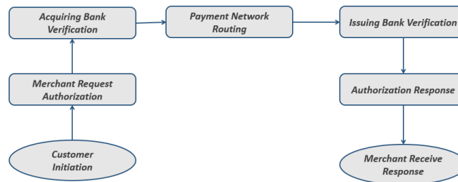
Fig. 3 Authorization Process
